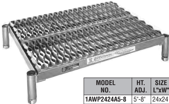
MODEL 1AWP2424A5-8
