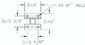
BASE BOLT PATTERN FOR 4" & 5" COLUMNS
