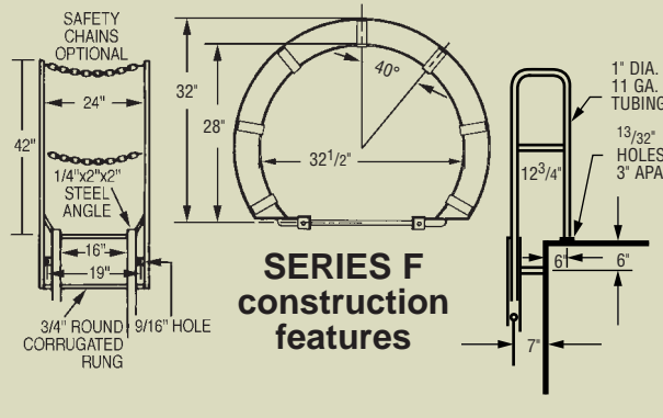
11 RUNG WITH WALK-THRU F11W
