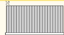
R_HE-G02203 22 groove trays
